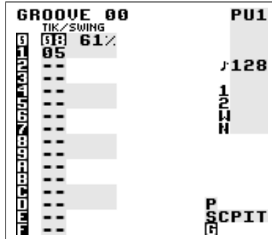
Figure 2.13: Swing Example
