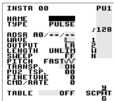
Figure 2.4: Instrument Screen
