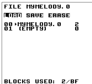
Figure 2.18: File Screen
