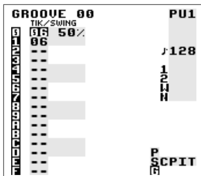
Figure 2.12: Groove Screen
