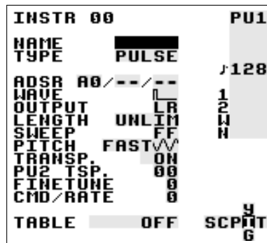
Figure 1.4: Instrument Screen
