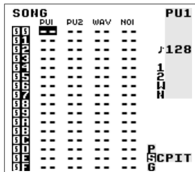
Figure 1.1: Song Screen
