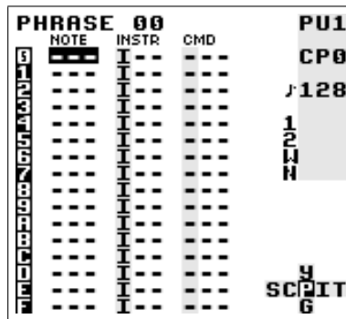
Figure 1.3: Phrase Screen
