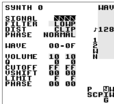
Figure 2.14: Synth Screen
