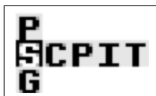
Figure 1.2: Screen Map
